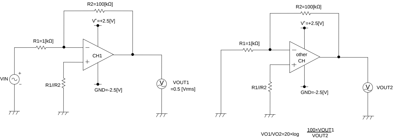
Fig.101 Measurement Circuit3
