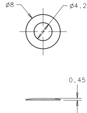
BELLEVILLE WASHER
