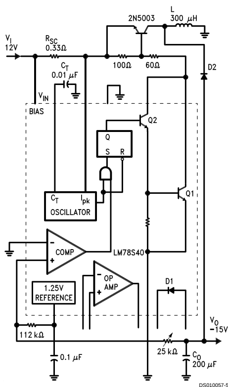
FIGURE 3. Typical Inverting Regulator and Operational Performance ( T_A = 25^\circ\text{C} )
