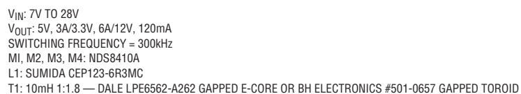
Figure 12. LTC3707 High Efficiency Low Noise 5V/3A, 3.3V/5A, 12/120mA Regulator
