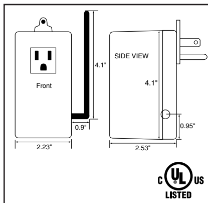
Figure 1: Package Dimensions
