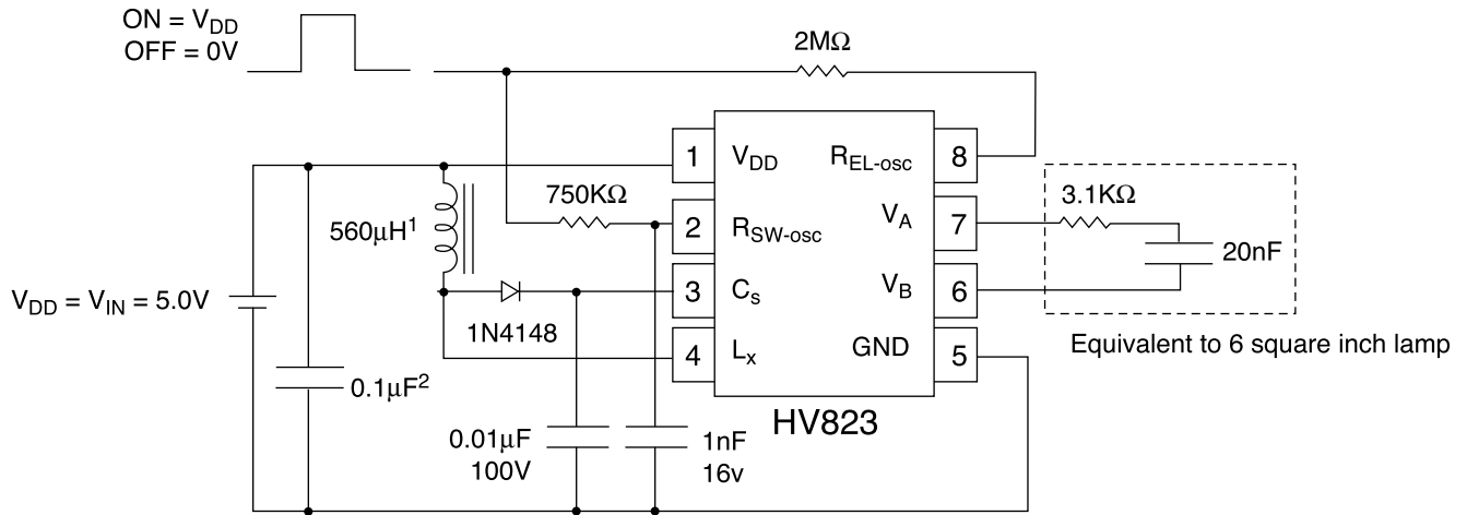
Figure 2: Typical 5.0V Application
