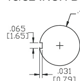
15/32 INCH BUSHING
