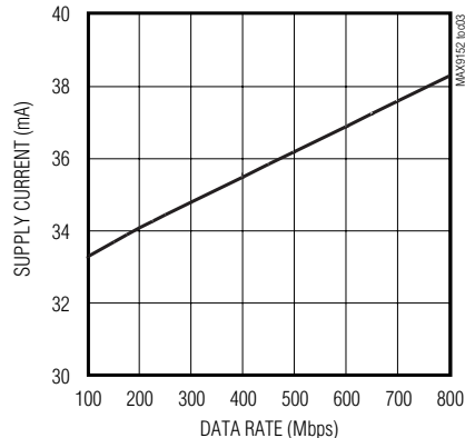
SUPPLY CURRENT vs. DATA RATE
