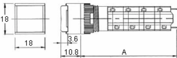
Mounting Dimensions
