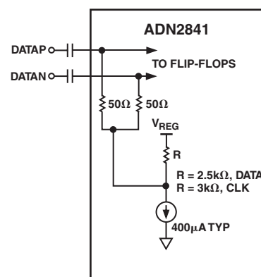
Figure 4. AC Coupling of Data Inputs
