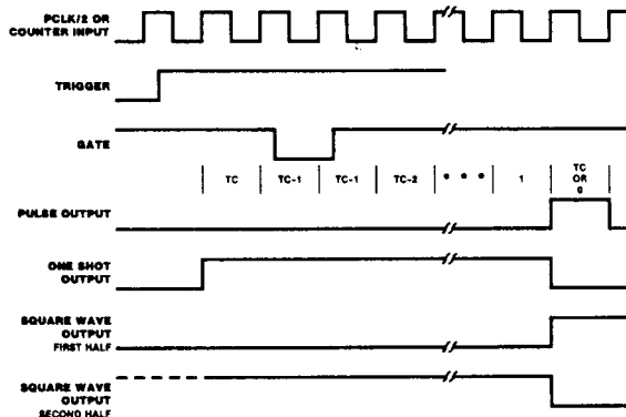
Figure 10. Counter/Timer Waveforms
