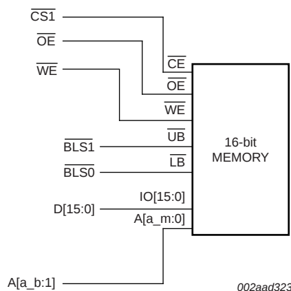
Fig 22. Booting from a single 16-bit memory chip
