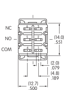
Double Pole
