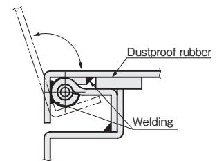
Installation Layout
