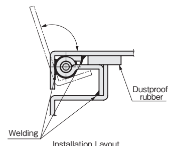
Installation Layout
