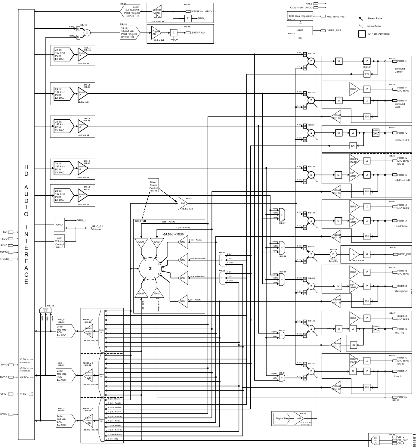
Figure 1. Block Diagram
