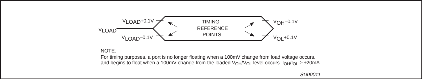
Figure 38. Float Waveform
