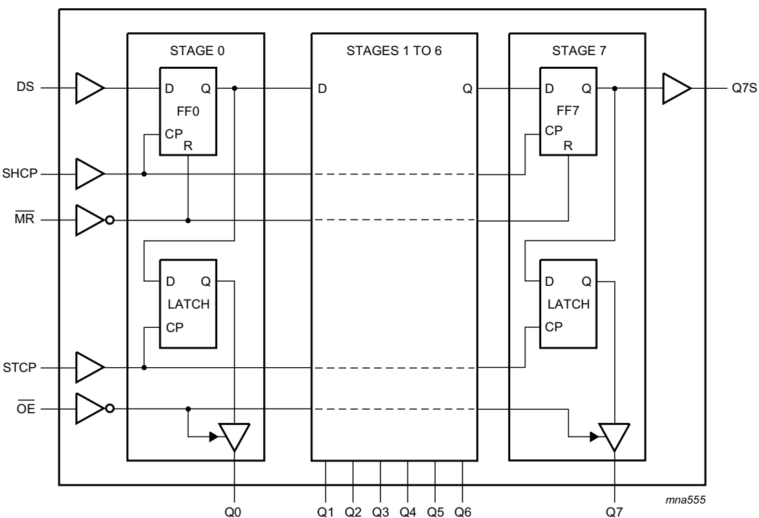
Fig 3. Logic diagram
