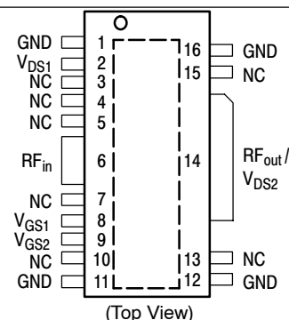
Figure 2. Pin Connections
