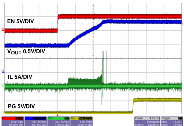
FIGURE 26. SOFT-START WITH PRE-BIASED V_{IN}
