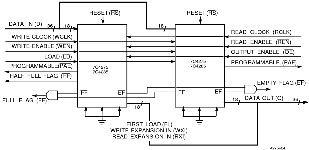
Figure 1. Block Diagram of 32K x18/64K x 18 Synchronous FIFO Memory Used in a Width Expansion Configuration.
