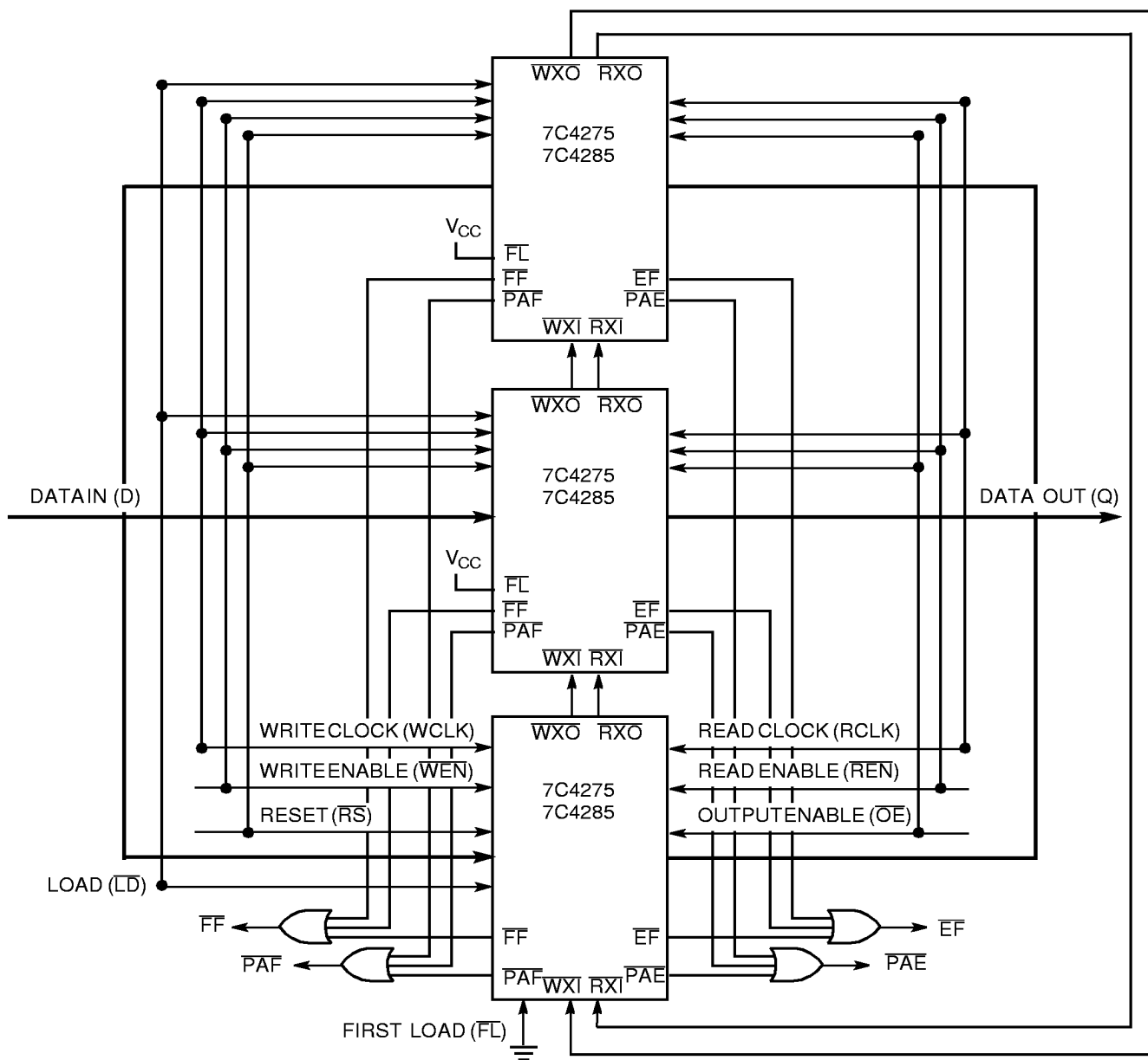
Figure 2. Block Diagram of 32Kx18/64Kx18 Synchronous FIFO Memory with Programmable Flags used in Depth Expansion Configuration.
