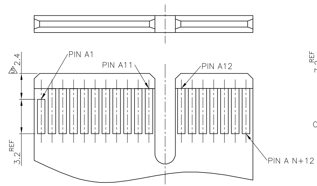
MODULE LAYOUT(MATING PART ONLY)
