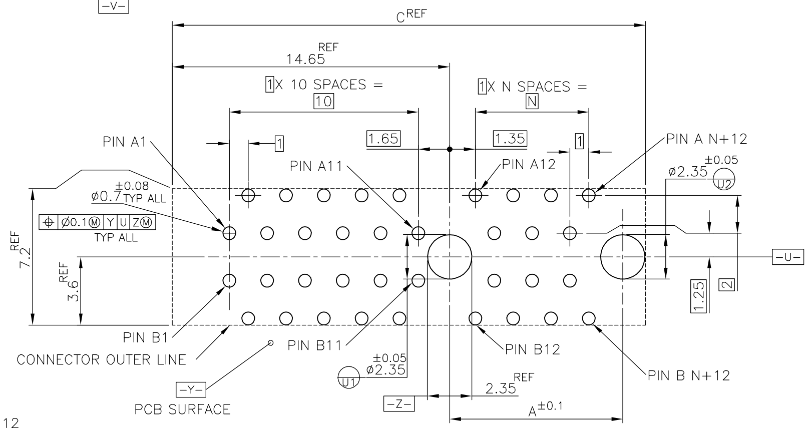
PCB PATTERN LAYOUT
