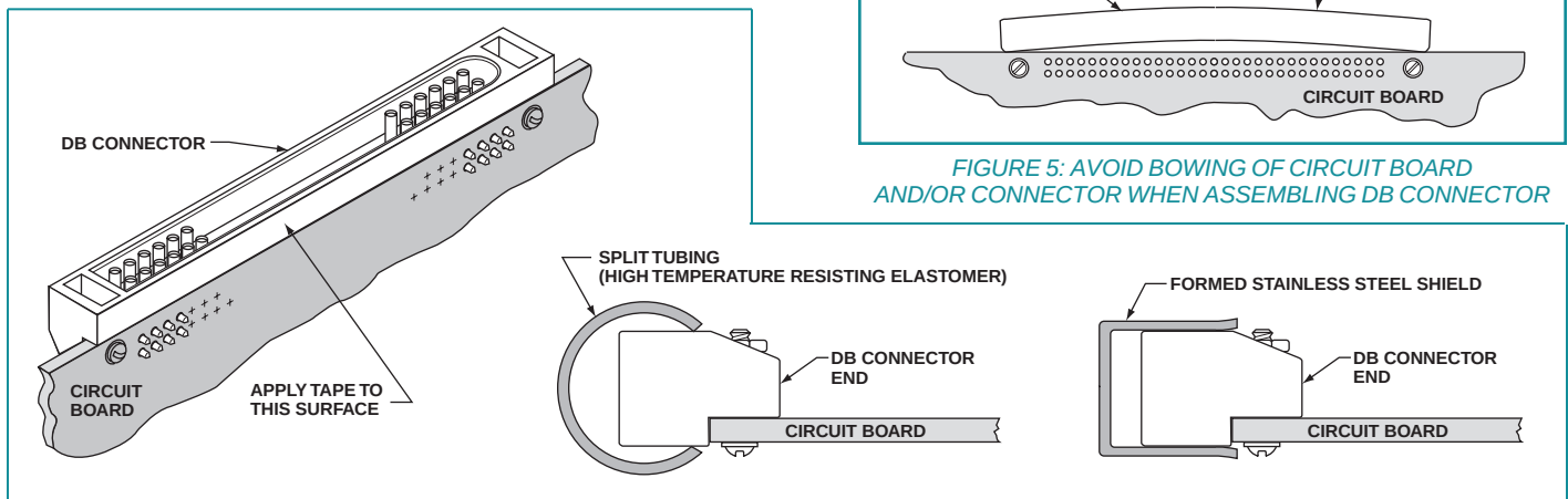
FIGURE 5: AVOID BOWING OF CIRCUIT BOARD AND/OR CONNECTOR WHEN ASSEMBLING DB CONNECTOR
