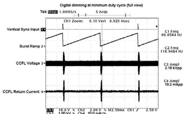
Figure 4 – 2% Burst Duty Cycle
