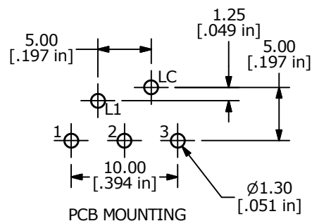
CIRCUIT LAYOUT
