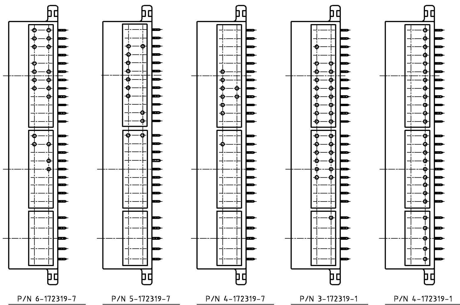
A方向から見た金めっき配置図 (LAYOUT OF GOLD PLATING CONTACT VIEW FROM "A" DIRECTION)
