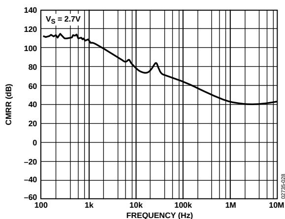
Figure 30. CMRR vs. Frequency at 2.7 V
