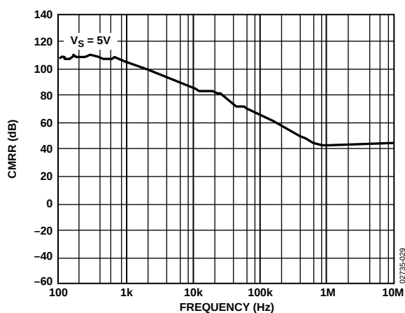
Figure 31. CMRR vs. Frequency at 5 V
