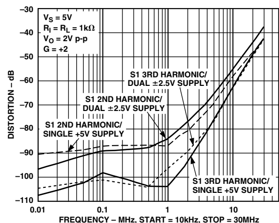
TPC 14. Harmonic Distortion vs. Frequency
