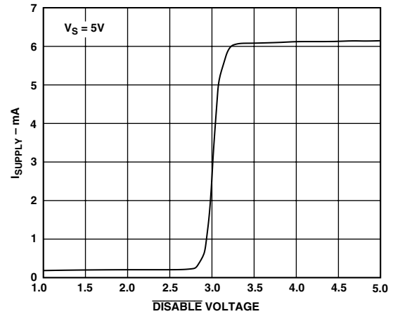
TPC 28. \overline{\text{DISABLE}} Voltage vs. Supply Current
