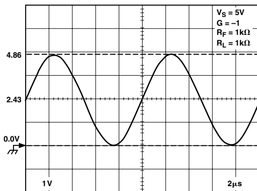
TPC 33. Output Swing
