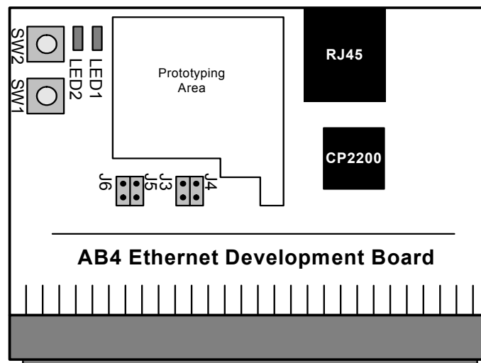
Figure 33. AB4 Ethernet Development Board
