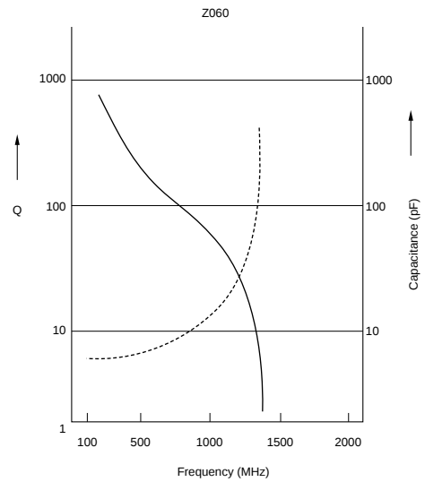
TZC3Z060
