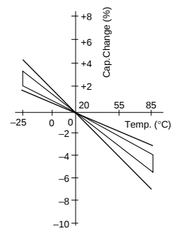
TZ03R121
