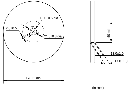
TZC3/TZW4/TZB4 Series
