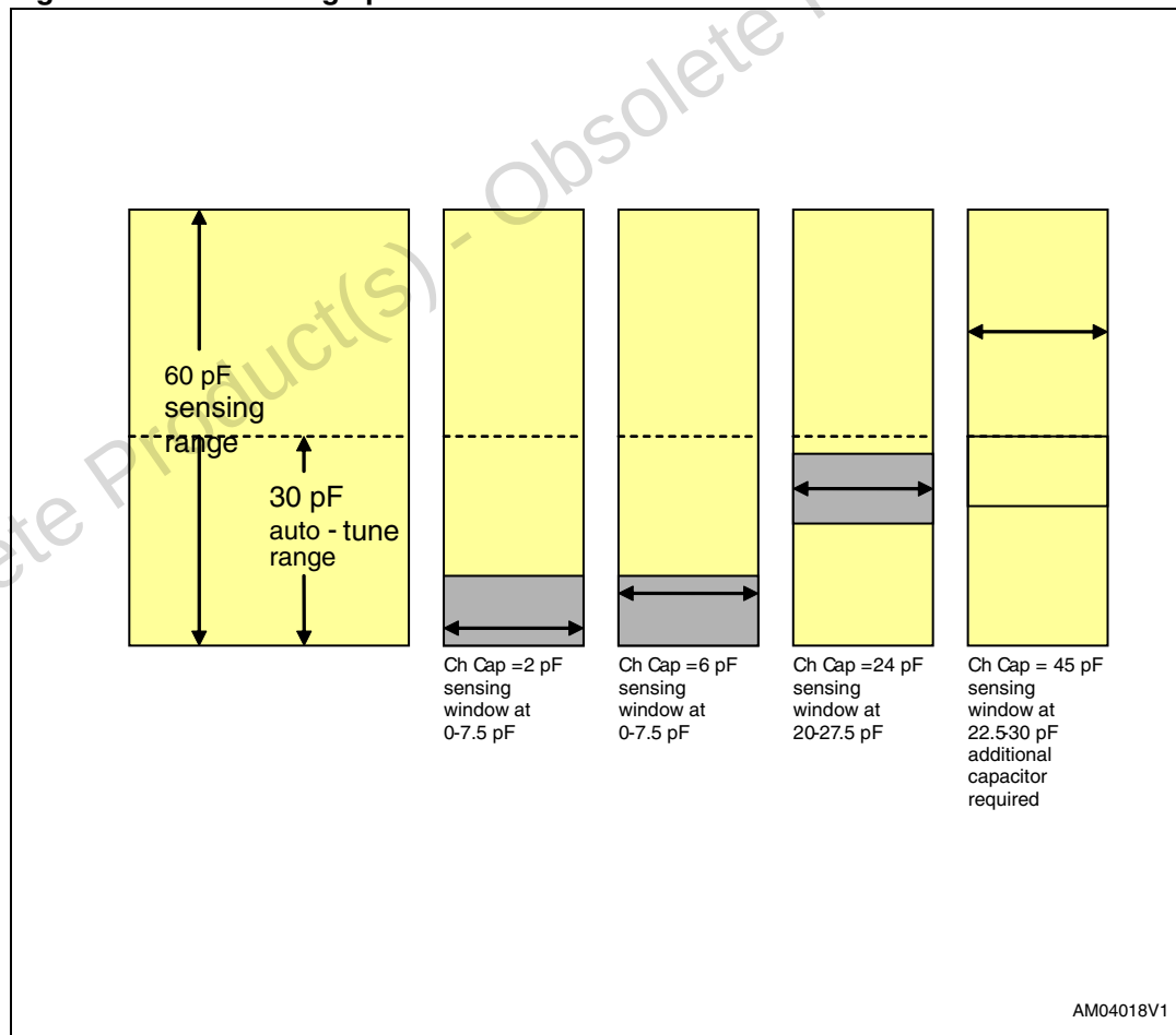
Figure 15. Auto-tuning operation
