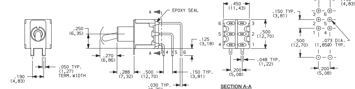
7201MD9AV2BE Vertical Actuation DPDT
