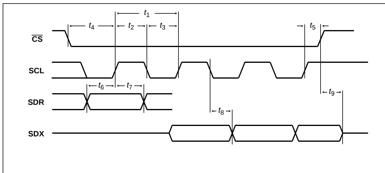
Figure 94 SCI Interface
