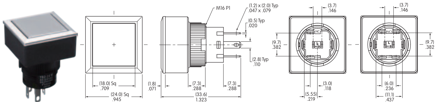
YB216CWSPW01-N-P
