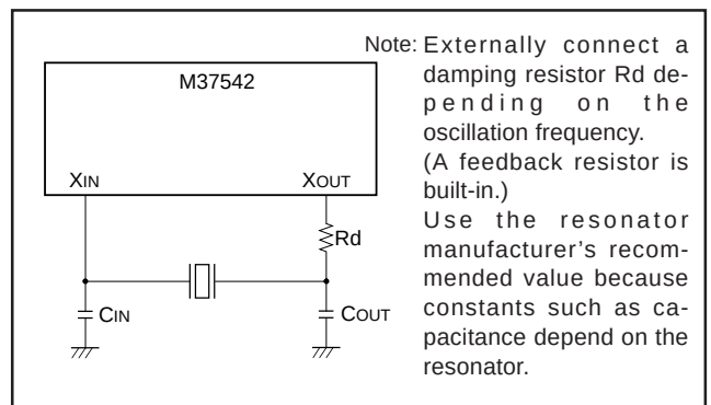
Fig. 74 External circuit of ceramic resonator
