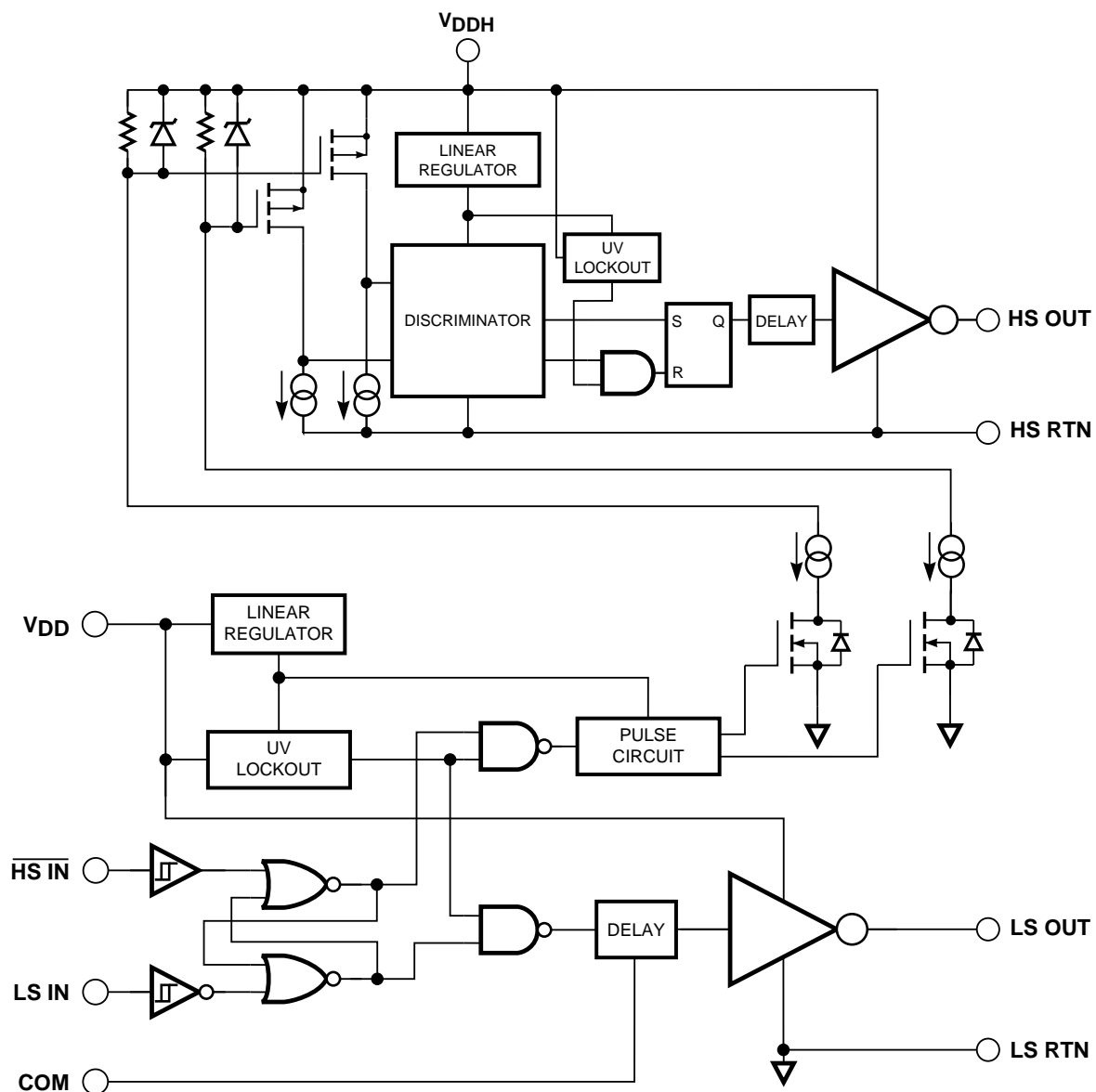
Figure 3. Functional Block Diagram of the INT100
