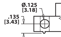
SIDE MOUNTING (S)
