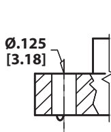
CLEARANCE HOLE (H)
