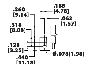
STRADDLE MOUNT (Q) Formerly (Z)
