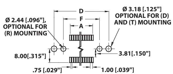
CONNECTOR SIDE (HF)
