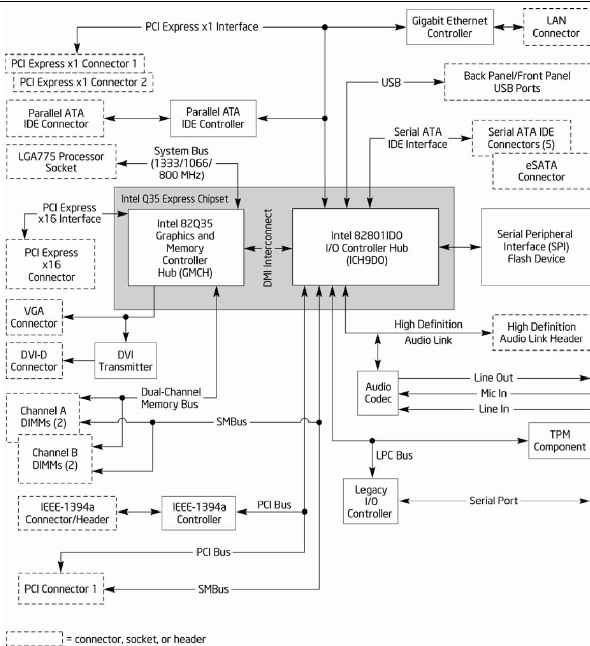
Figure 2. Block Diagram
