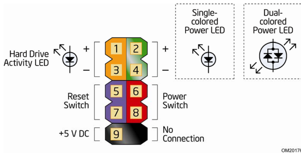
Figure 12. Connection Diagram for Front Panel Header
