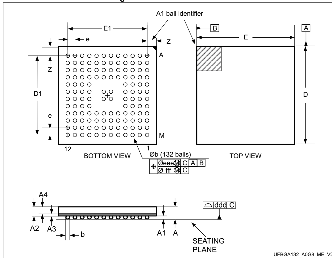
Figure 78. UFBGA132 outline
