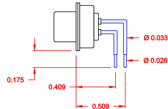
SIGNAL CONTACTS
