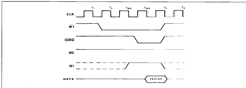
Figure 14 : Interrupt Acknowledge Timing.
