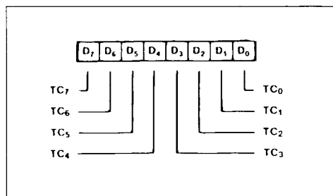
Figure 7 : Interrupt Vector Word.
