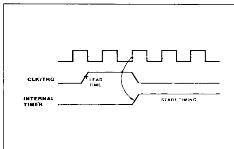
Figure 12 : Counter Mode Timing.
