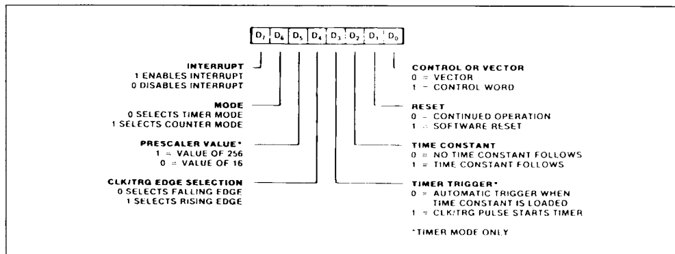
Figure 5 : Channel Control Word..
