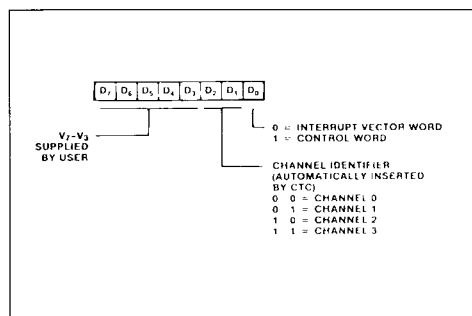
Figure 7 : Interrupt Vector Word.
