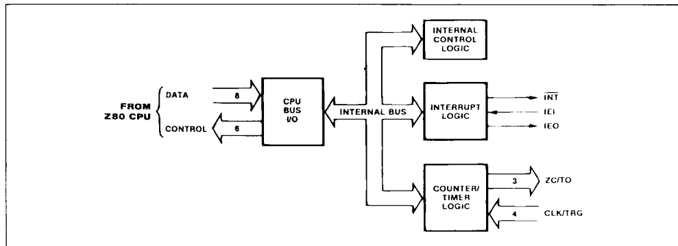
Figure 3 : Functional Block Diagram.
