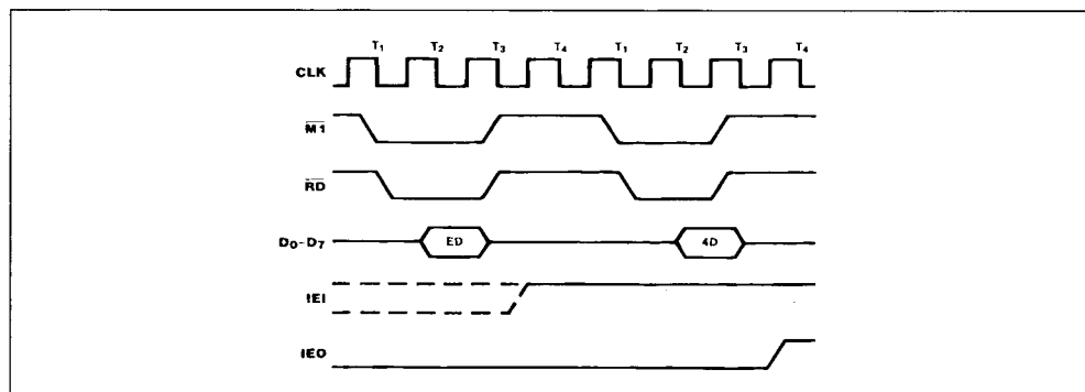
Figure 15 : Return From Interrupt Timing.
