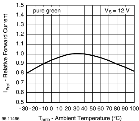
Fig. 25 - Relative Forward Current vs. Ambient Temperature
