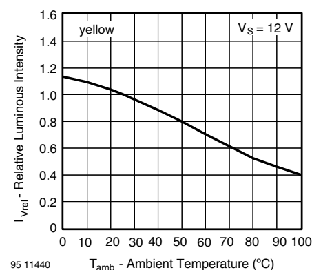
Fig. 16 - Relative Luminous Intensity vs. Ambient Temperature
