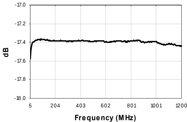
Coupling Forward (Pin 6 to 4)
