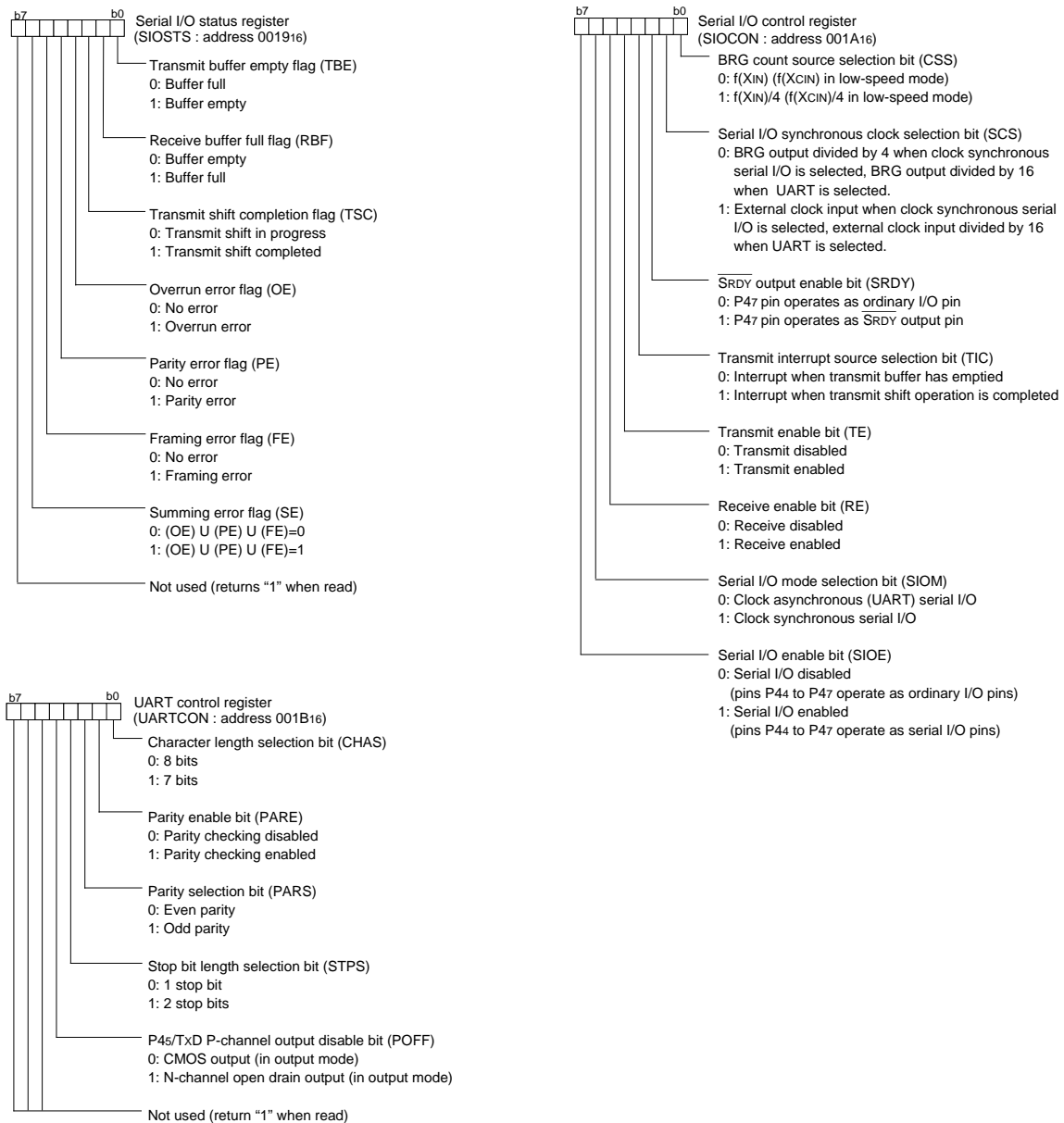
Fig. 30 Structure of serial I/O control registers
