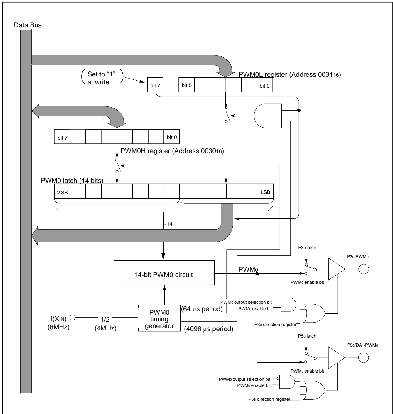
Fig. 23 PWM block diagram (PWM0)
