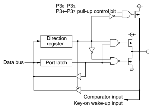
(5) Ports P3 2 –P3 7
