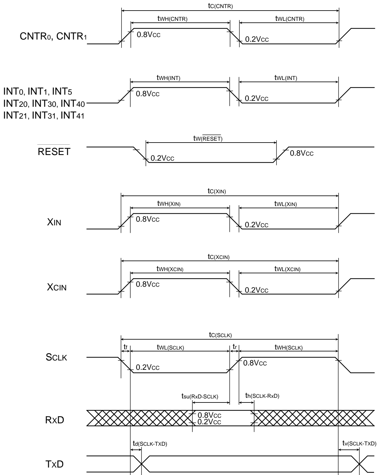
Fig. 84 Timing diagram
