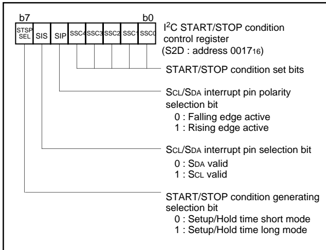
Fig. 41 Structure of I²C START/STOP condition control register
