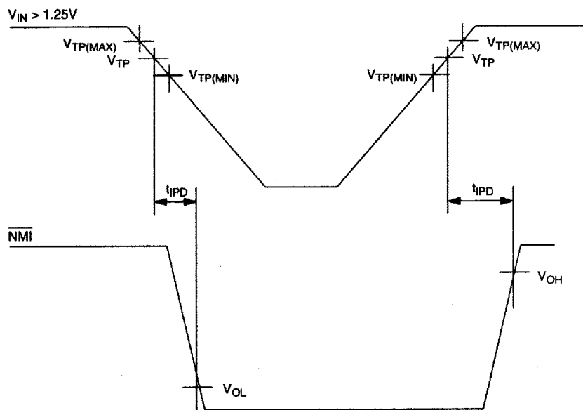
TIMING DIAGRAM: NON-MASKABLE INTERRUPT Figure 4
