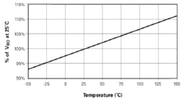
Figure SB4 - Breakover Voltage vs. Temperature
