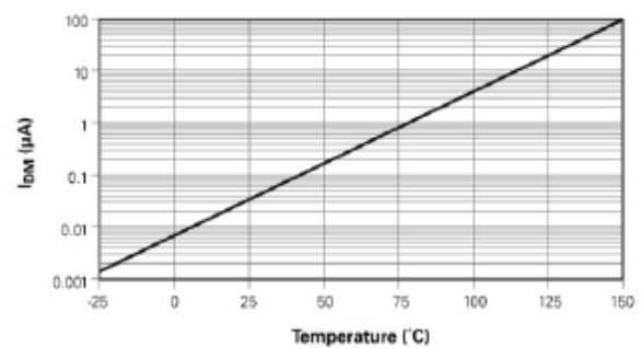
Figure SB6 - Off-state Current vs. Temperature
