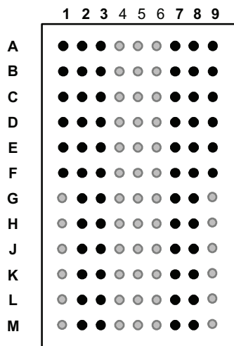
BGA Package Ball Pattern Top View
