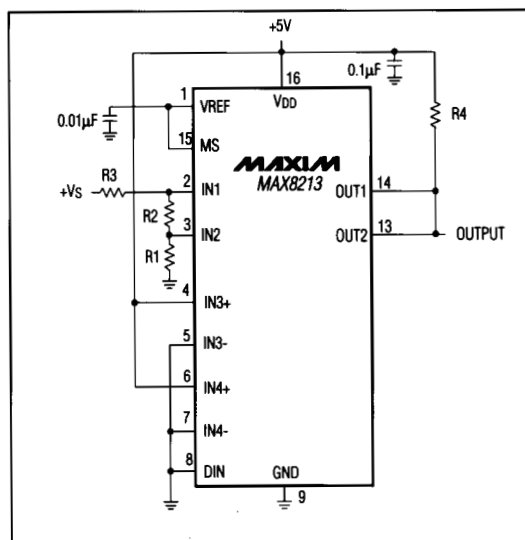
Figure 11. Window Detector
