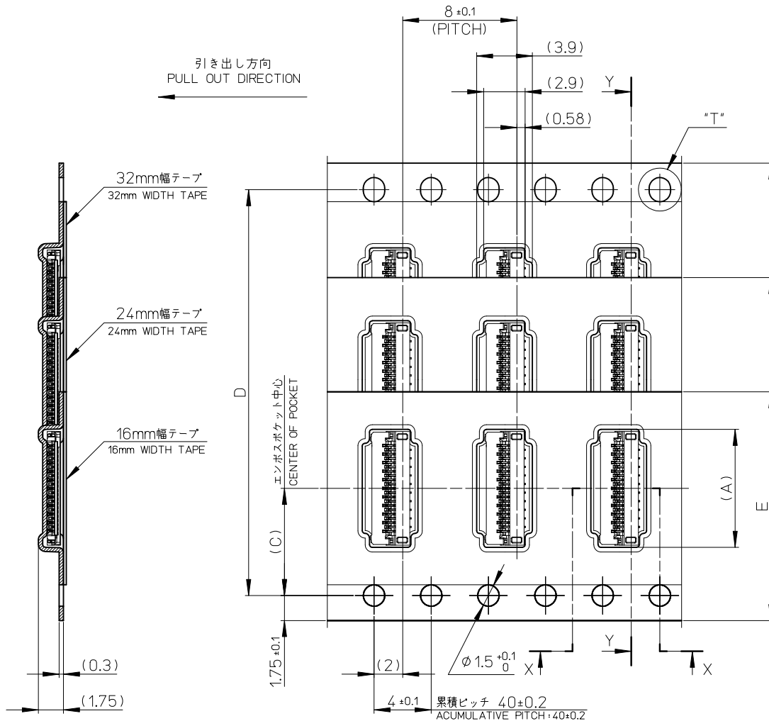
SECTION Y-Y
