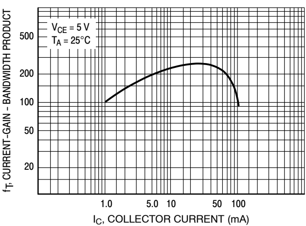
Figure 18. Current-Gain - Bandwidth Product
