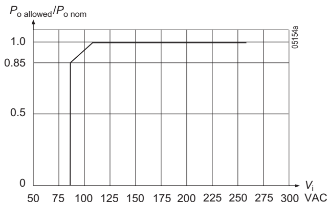
Fig. 3 Maximum allowed output power versus input voltage at T_A = 50^\circ\text{C} for LOK models operated in vertical position
